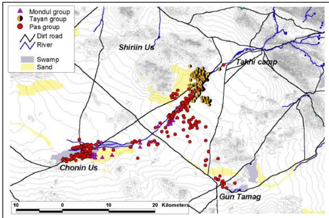
Fig. 3: Locations of the three Takhi groups monitored with GPS / ARGOS telemetry from January until July 2004.
