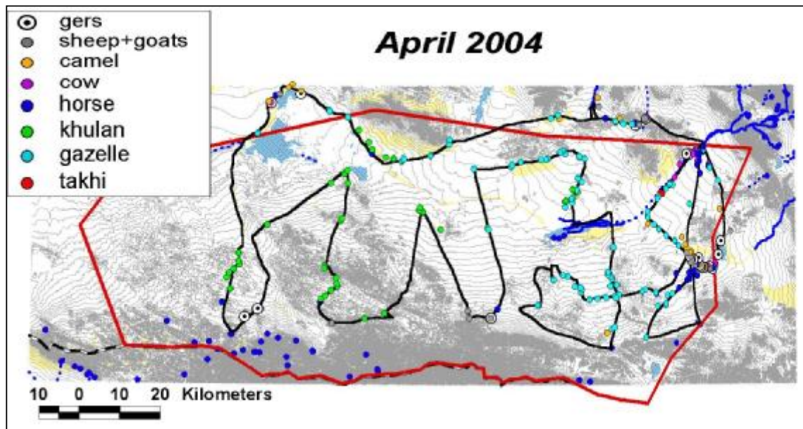
Fig. 10: Wild- and domestic ungulate observations on the wildlife count driven in April 2004.
