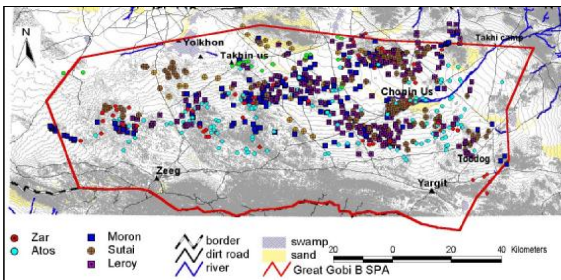
Fig. 8: Locations of 7 khulans monitored in the Gobi B National Park from July-November 2003.
