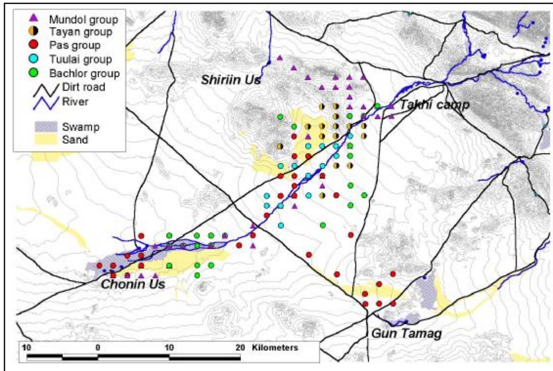
Fig. 4: Takhi observations by park rangers January – July 2004 based on a raster map with 2 x 2 km edge length.
