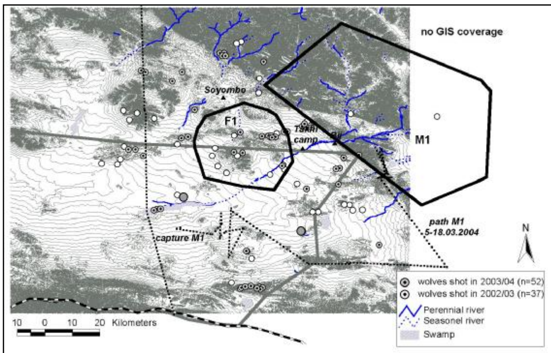
Fig. 7: Home ranges of the collared wolves Booro and Tzimtzik and the location of wolves killed in the eastern part of the Great Gobi B SPA from fall 2002 until spring 2004.
